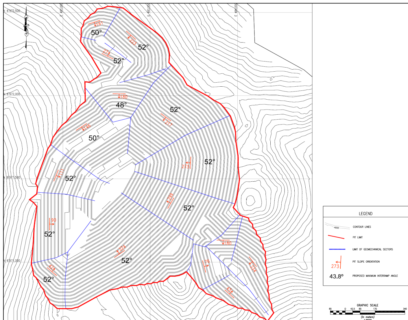
Figure 16-2: Geotechnical Sectors
