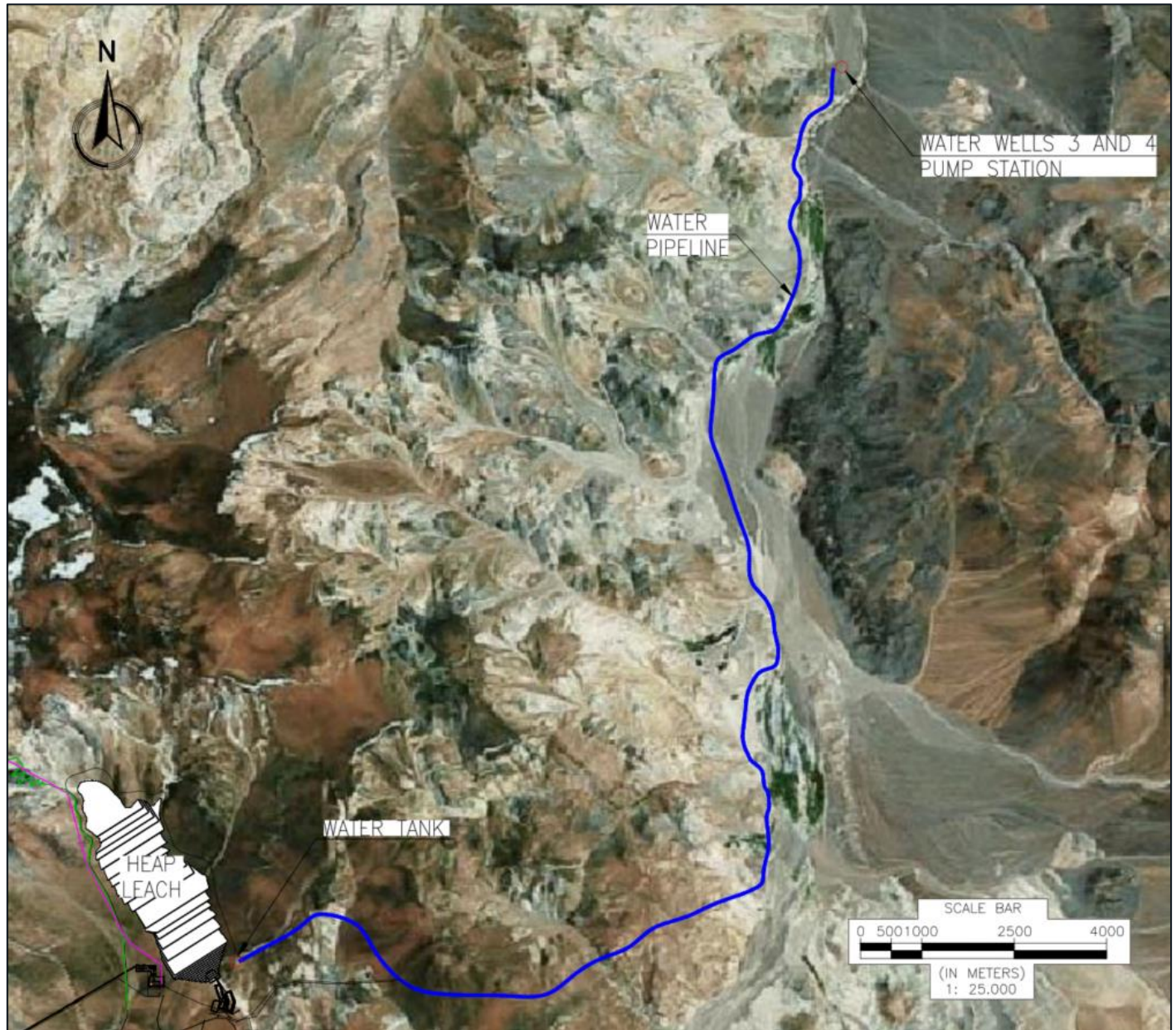
Figure 18-10: Pipeline Route
