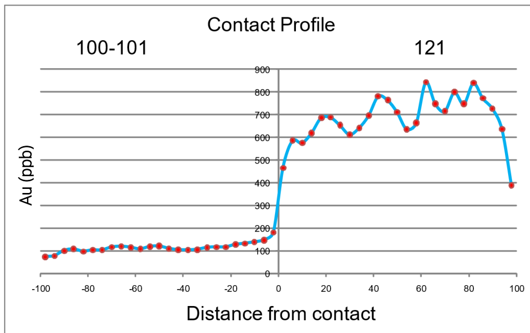
Figure 14-11: Contact Analysis, Dorado Oeste (Sur) Deposit, Domain 100/101 – 121
