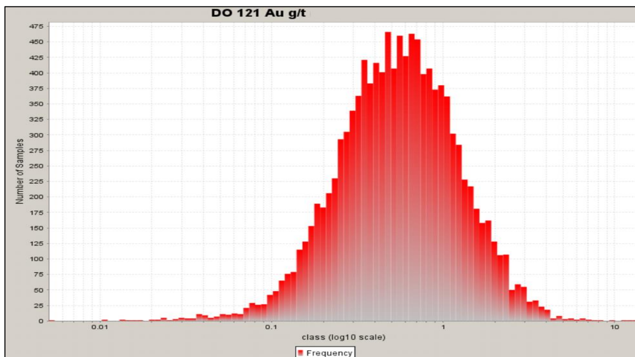
Figure 14-14: Frequency Log-normal Histogram of the Gold Values Contained Within the DO (South) Domain 121
