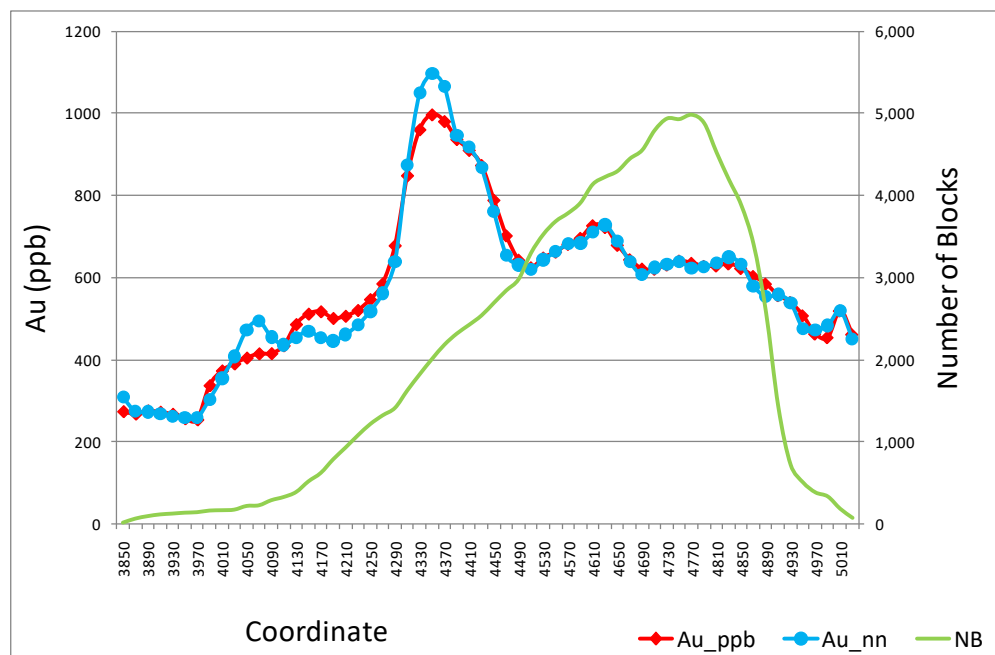
Figure 14-28: Drift Analysis for the DO (Sur) Domain (Code 121) (Bench data are presented on the y-axis while cross-sectional data are presented on the x-axis)
