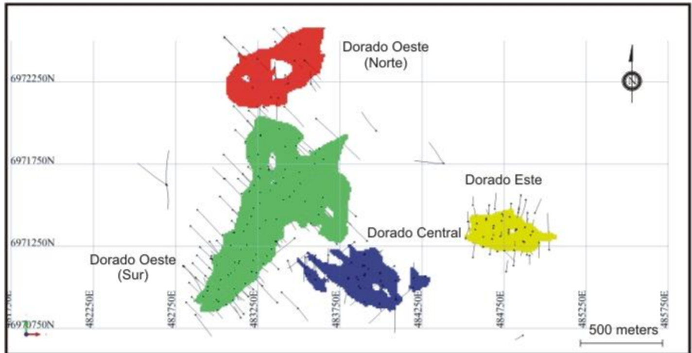
Figure 10-1: Plan View of the Drill Hole Coverage and Gold Deposits of the Dorado Sector, Volcan Property
