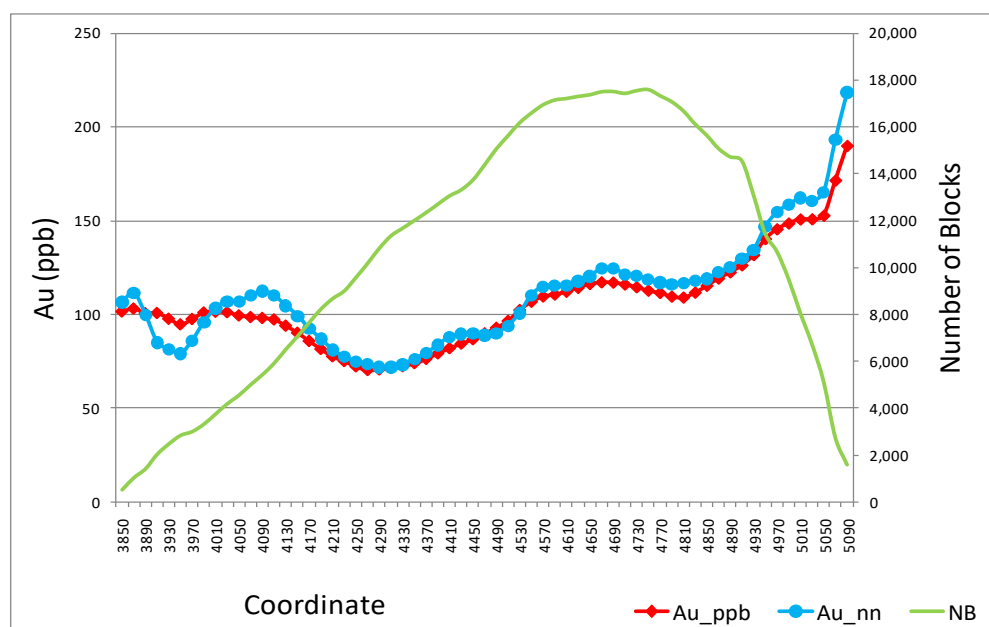
Figure 14-29: Drift Analysis for the DO Domain (Code 100/101) (Bench data are presented on the y-axis while cross-sectional data are presented on the x-axis)
