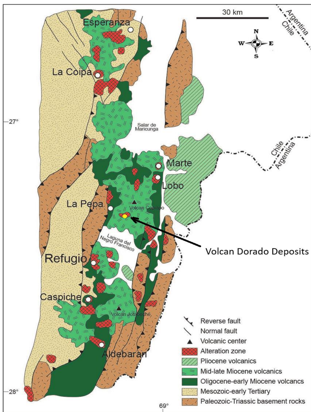
Figure 7-1: Generalized Map of Regional Geology
