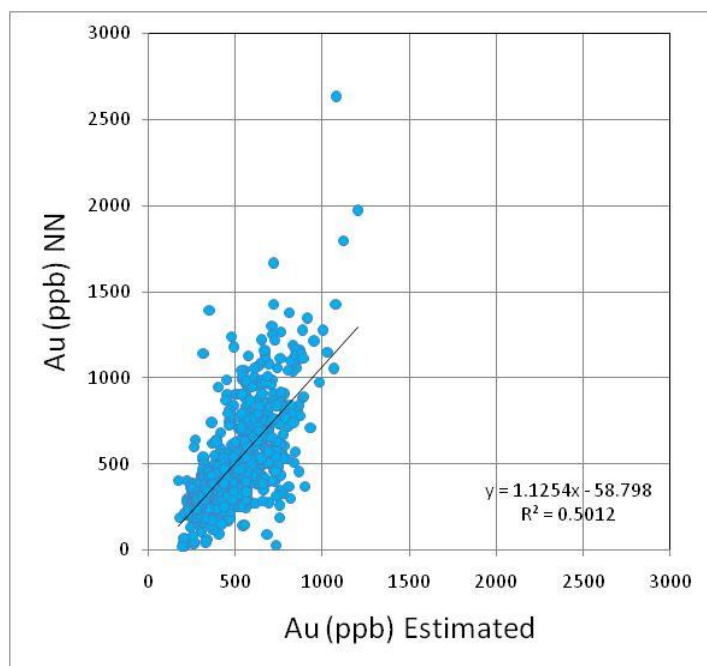
Figure 14-30: Dispersion Graph for DO (Norte 110/111), All Samples
