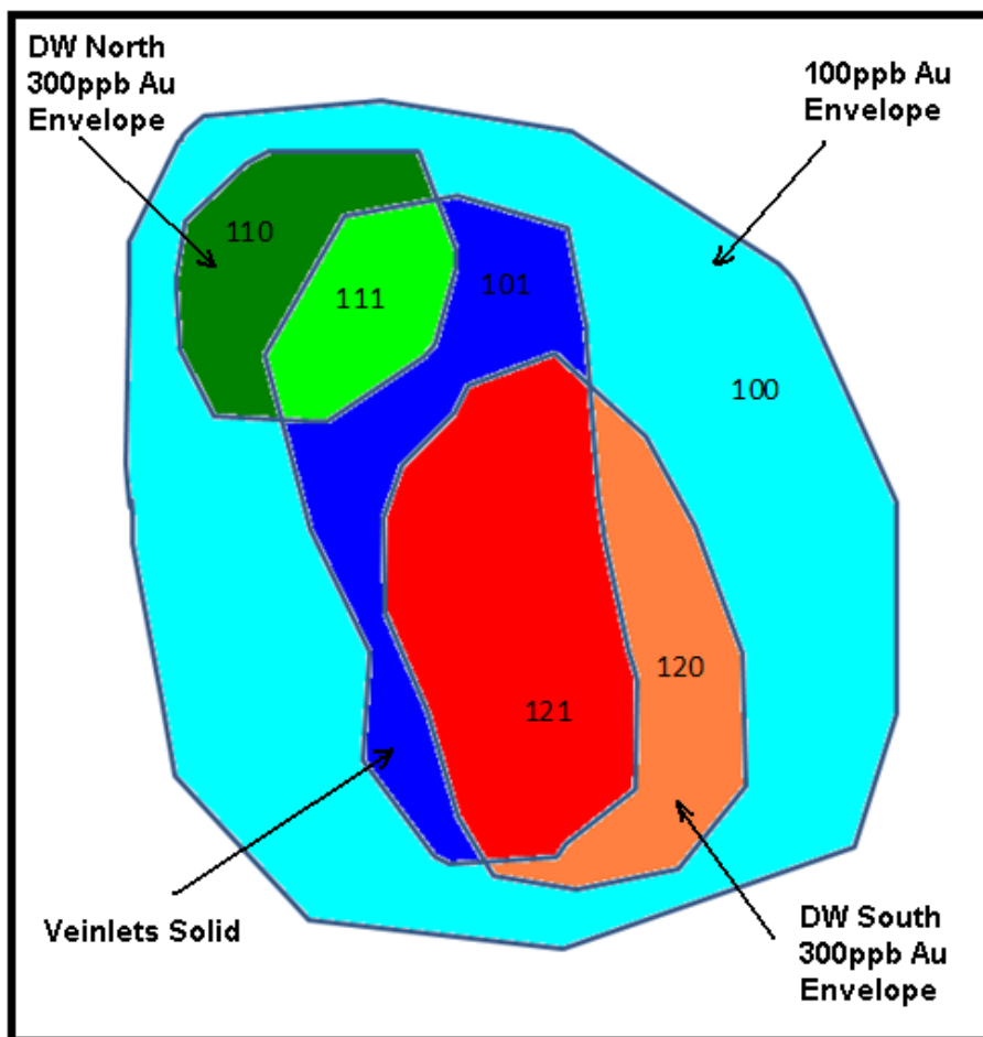
Figure 14-3: Dorado Oeste Deposit Domains - Graphical Schematic Representation (Not to Scale)
