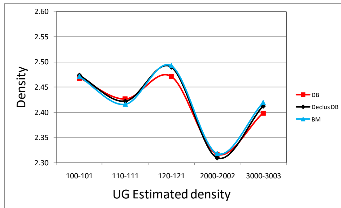
Figure 14-18: Graphical Comparison of Density – Block Model Estimates and Samples
