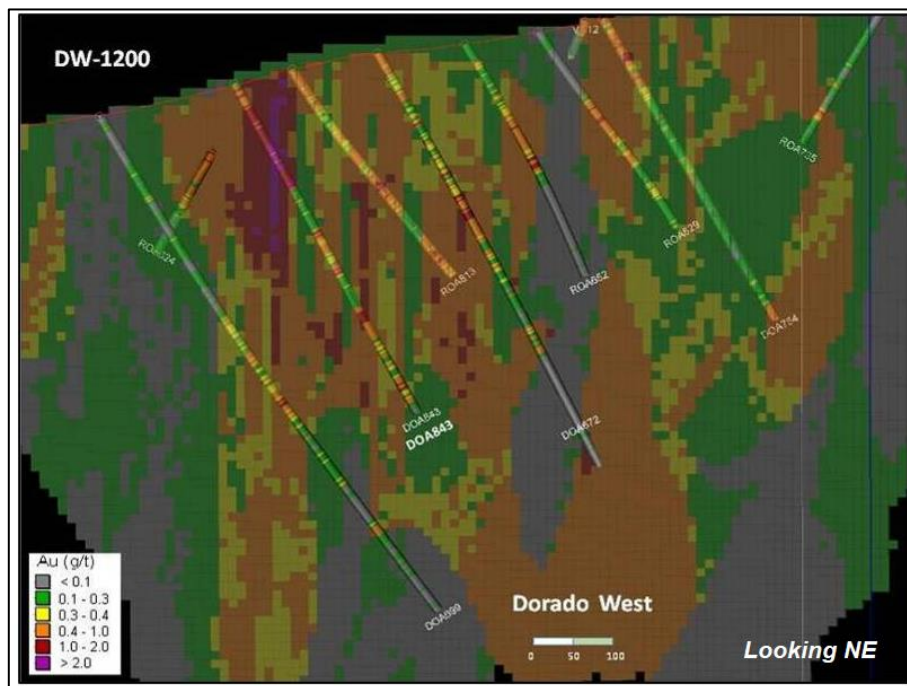
Figure 10-4: Cross-Section through Section Line DO-1200 Illustrating the Drill Holes and Gold Grade (g/t). Refer to Figure 10-2.
