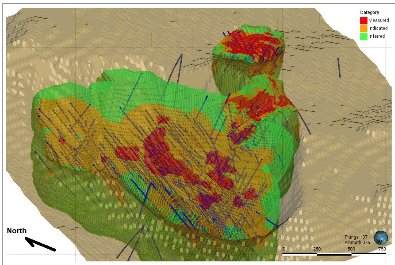
Figure 14-36: Isometric View of the Volcan Block Model Categorization
