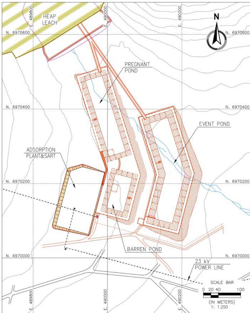
Figure 18-9: Platforms and Ponds
