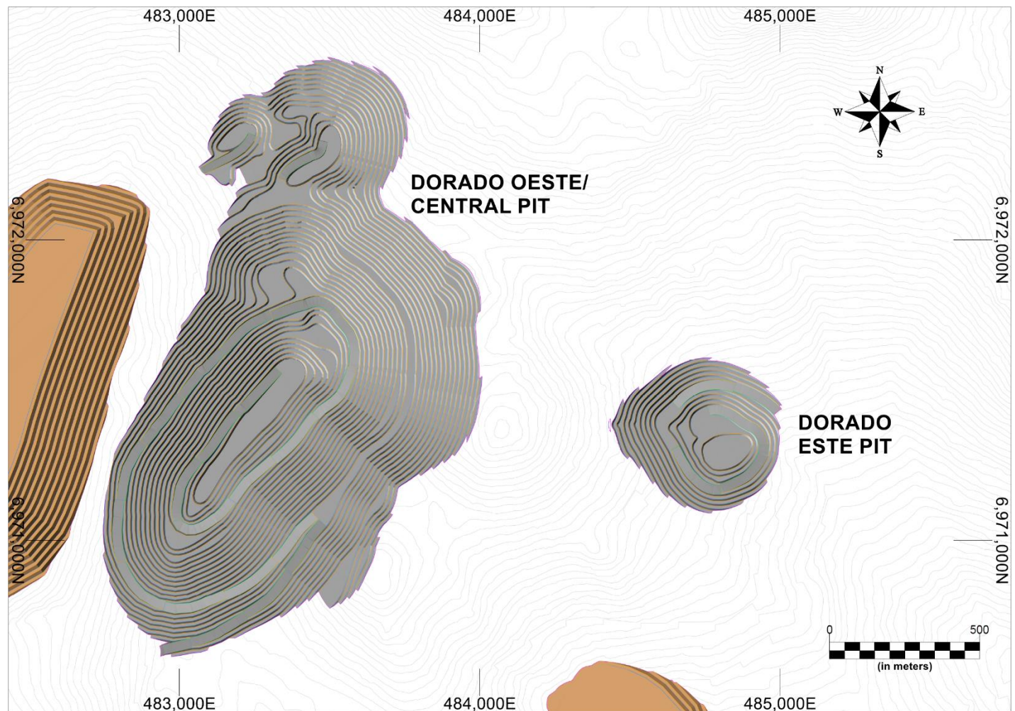
Figure 16-4: Final Pit Design
