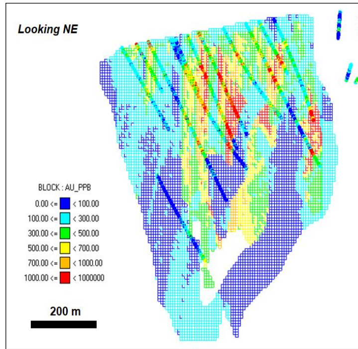
Figure 14-25: DO - Main Body – North End – Vertical Section
