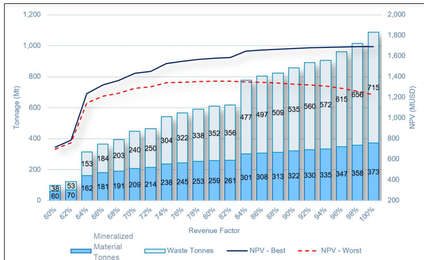
Figure 16-3: Pit Optimization Results
