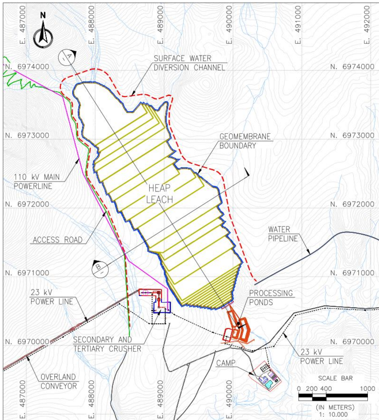
Figure 18-6: Heap Leach Pad – Plan View
