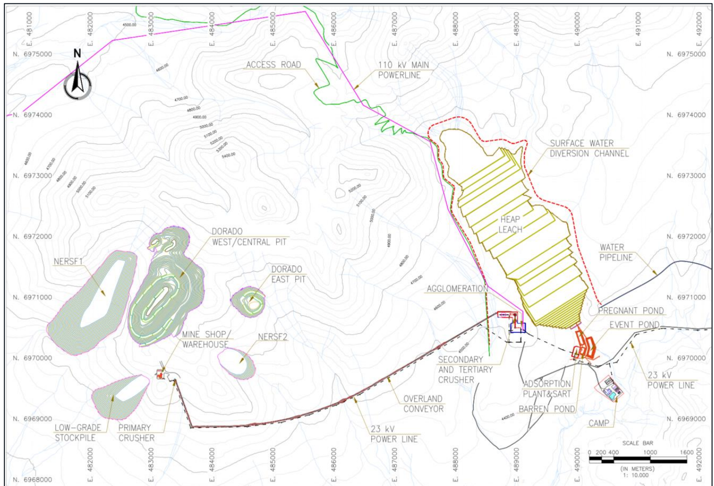
Figure 18-1: Overall Site Layout
