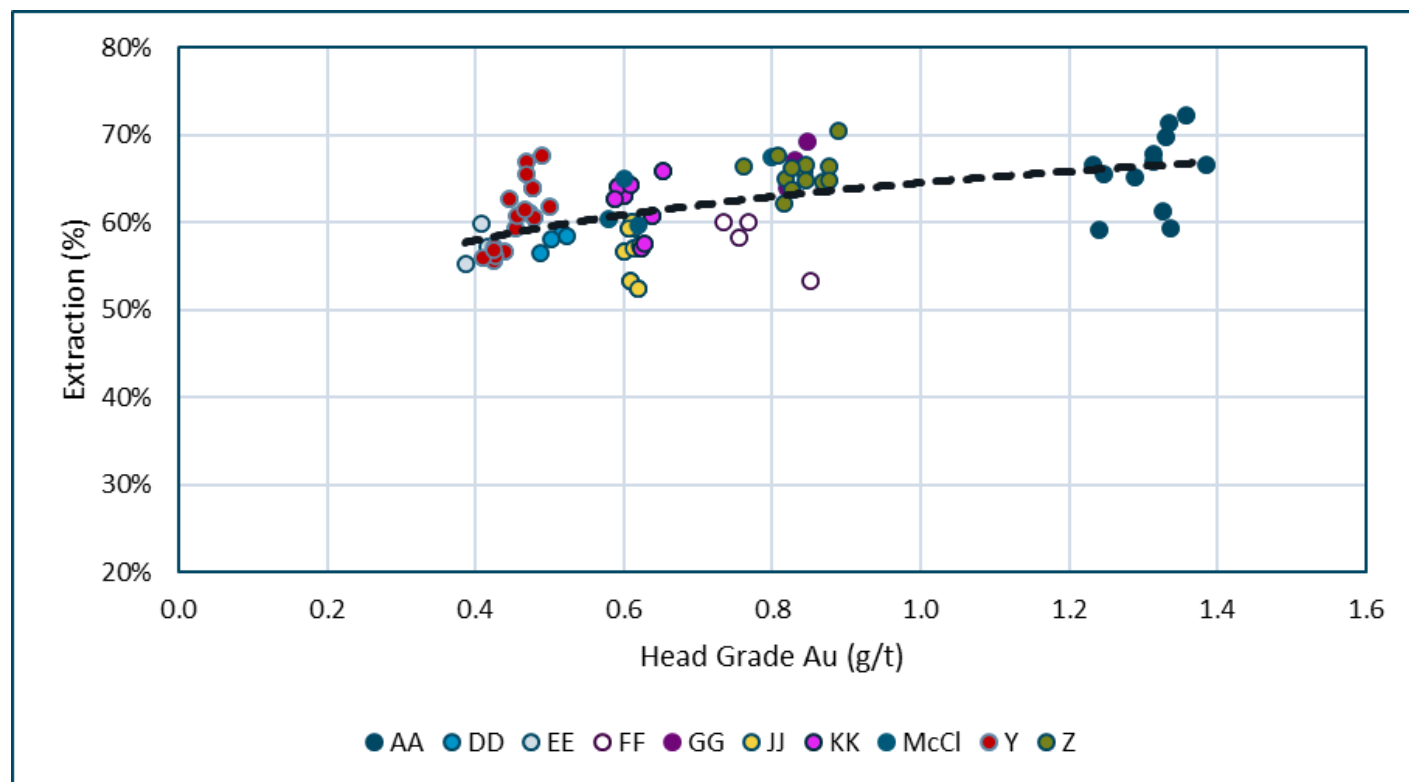
Figure 13-2: Gold Leach Recovery vs Head Grade for All Tests
