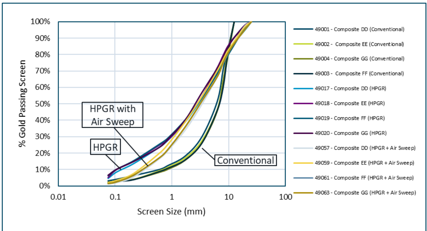
Figure 13-1: Gold Distribution by Size and Pre-treatment
