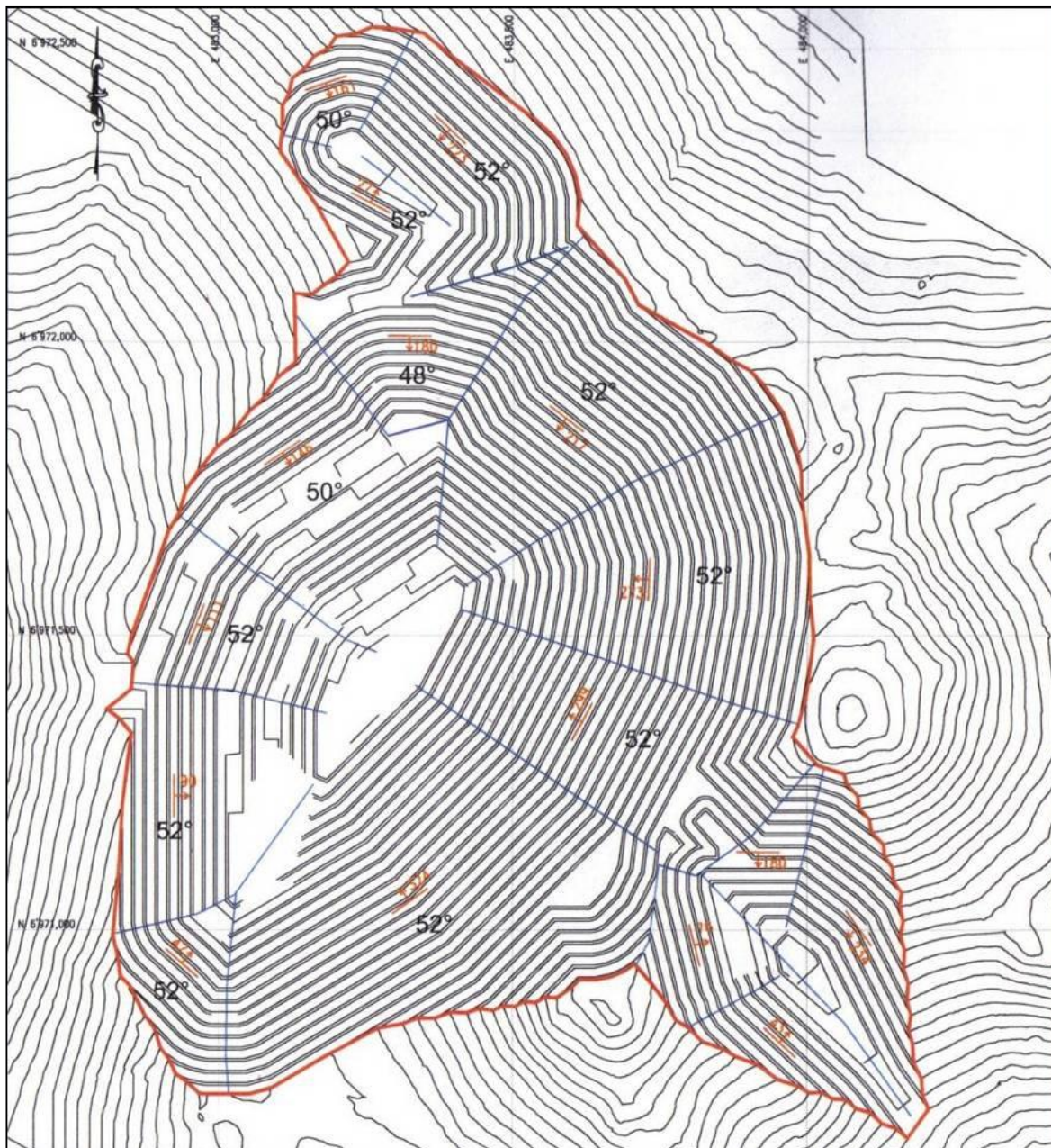
Figure 14-33: Preliminary Overall Wall Slope Sectors, Dorado Area Open Pits, Volcan Project
