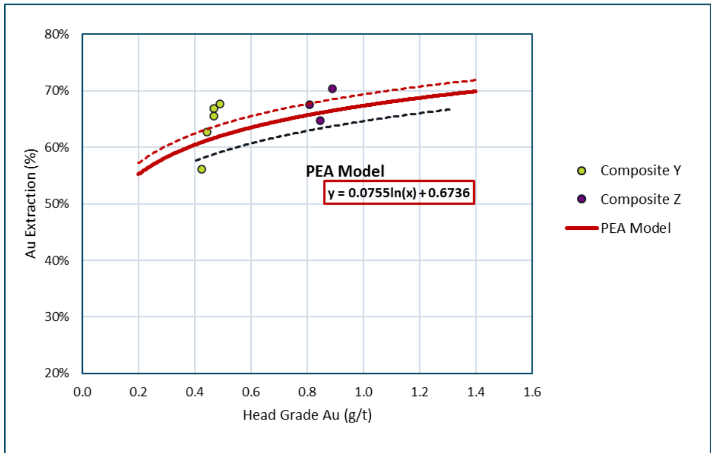
Figure 13-5: PEA Recovery Model – HPGR, 3.2 N/mm 2 pressure, fines retained
