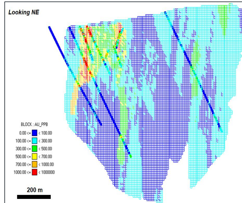
Figure 14-26: DO - Northern Body – GU 110 – 111 – Vertical Section
