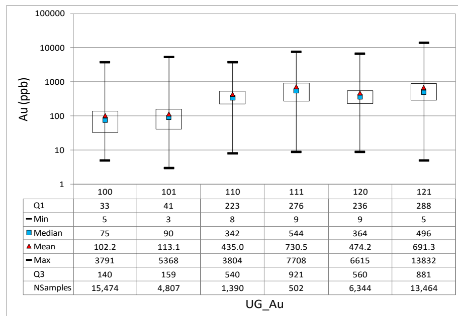
Figure 14-7: Box-and-Whisker Plot of Gold Assays Contained Within the Geological Domains (Columns), Excluding Ungrouped Weights
