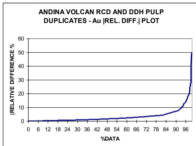
Figure 11-3: Results for the Pulp Duplicate Samples, Phase VI Exploration Program
