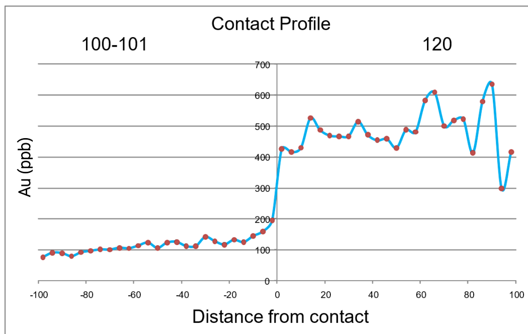
Figure 14-10: Contact Analysis, Dorado Oeste (Sur) Deposit, Domain 100/101 – 120
