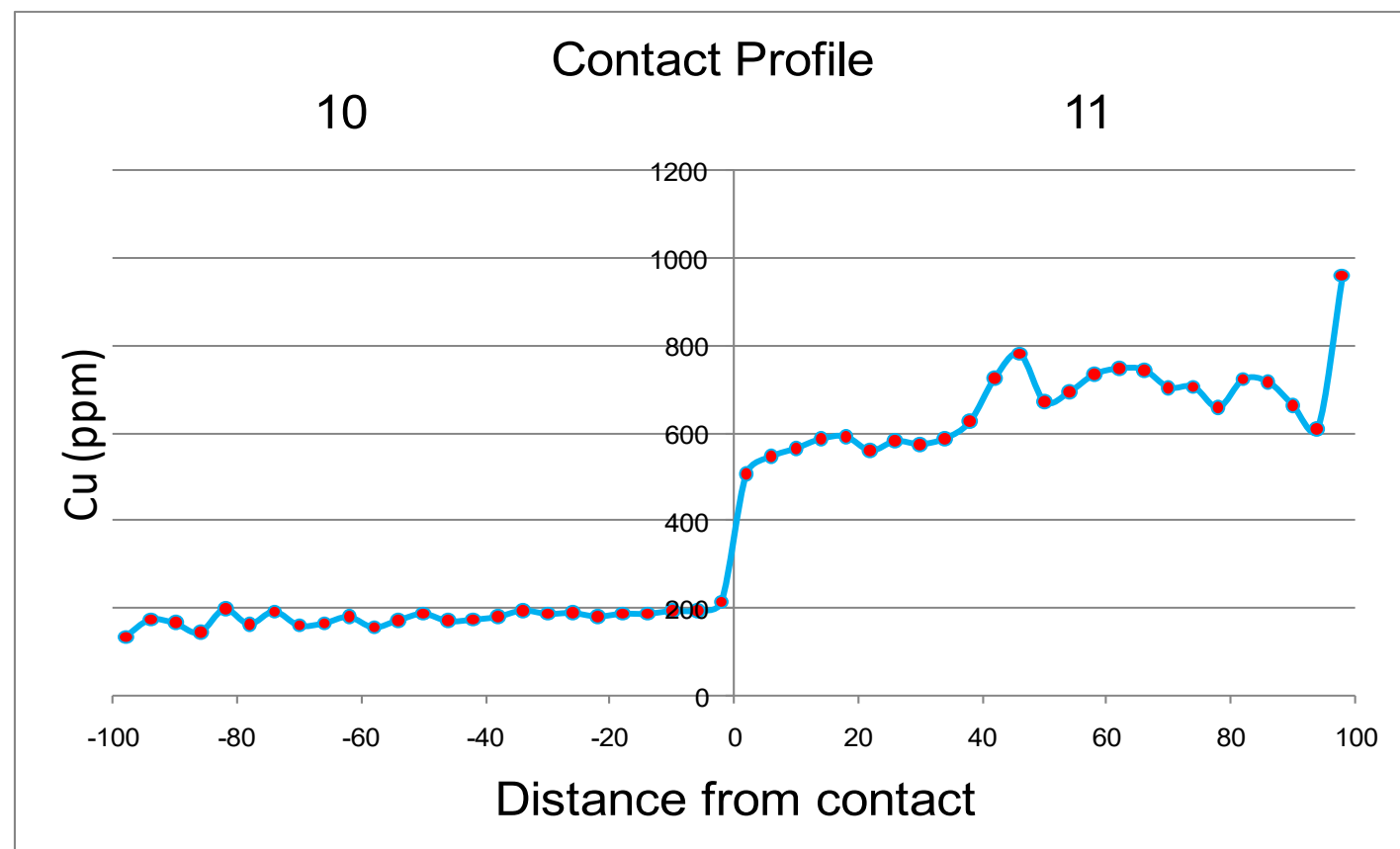
Figure 14-13: Contact Analysis, Dorado Oeste (South) Deposit, Domain 10 – 11
