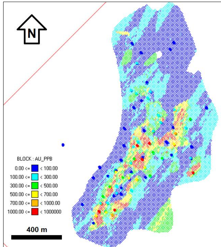
Figure 14-19: Bench Plan 4505, Dorado Block Model
