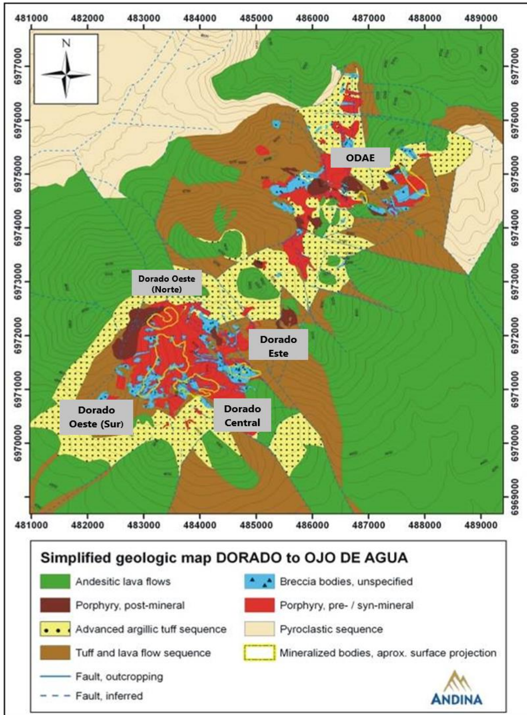
Figure 7-2: Simplified Geological Map of the Dorado to Ojo de Agua Este (ODAE) of the Volcan Property (Dorado Deposits outlined at bottom left, ODAE outlined at top right)
