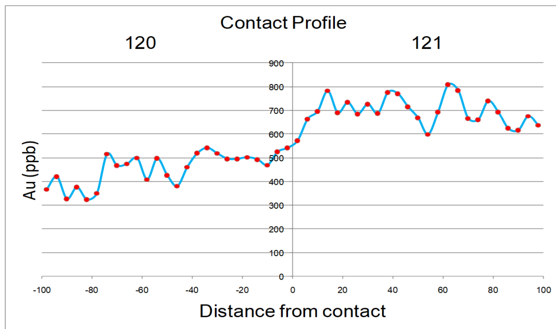
Figure 14-12: Contact Analysis, Dorado Oeste (Sur) Deposit, Domain 120 – 121
