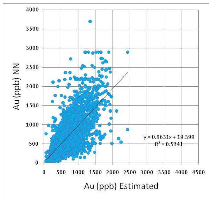
Figure 14-32: Dispersion Graph for DO (Sur, 121), All Samples
