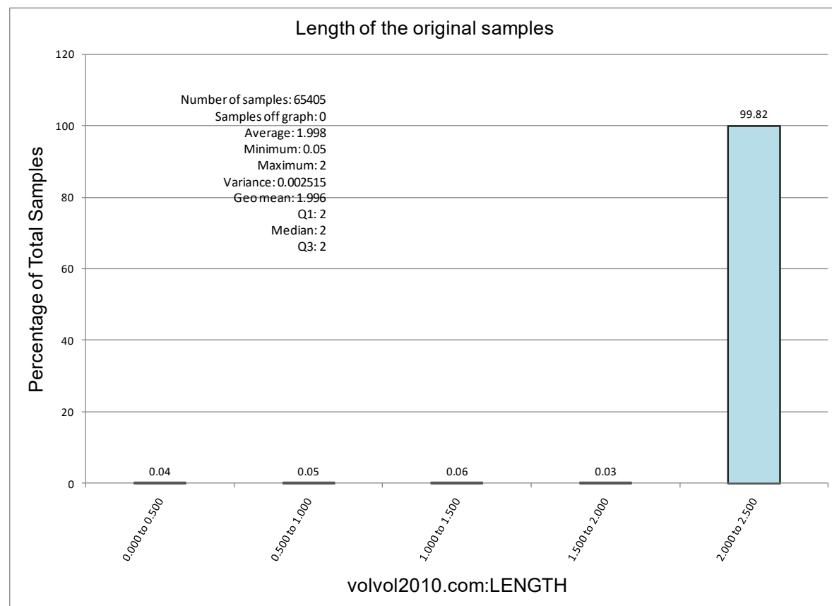
Figure 14-6: Histogram of Raw Sample Lengths, Volcan Project
