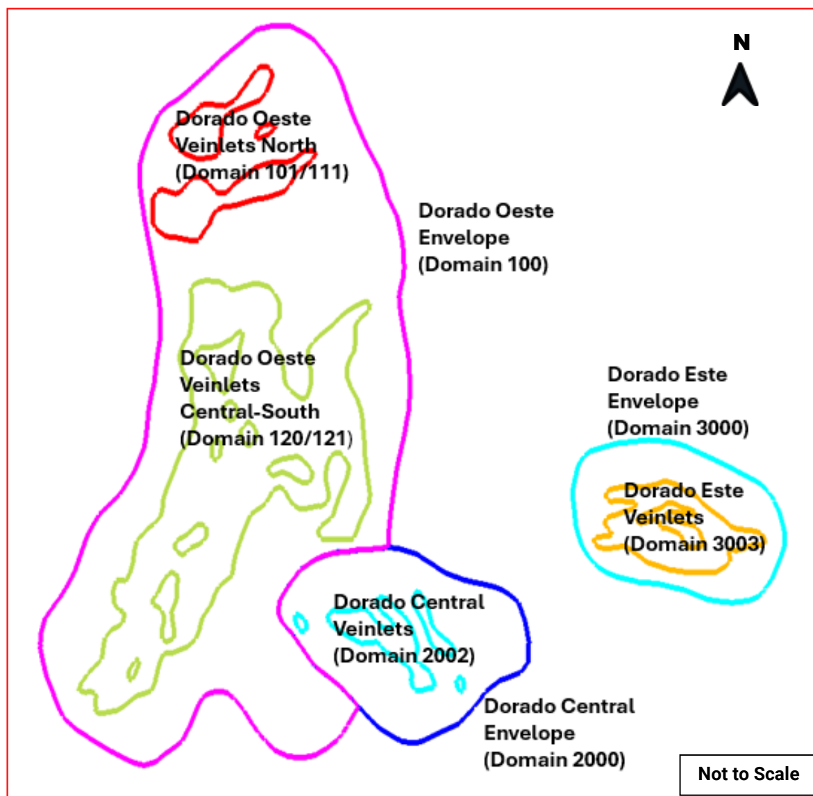
Figure 14-5: Plan View of the 4705 Bench Showing the Various Domain Outlines, Volcan Project
