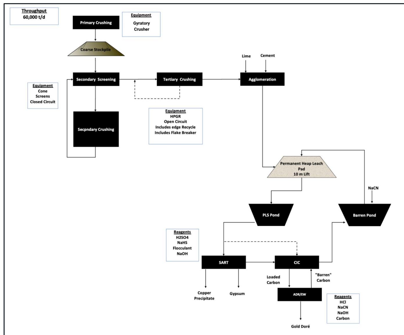
Figure 17-1: Process Flowsheet
