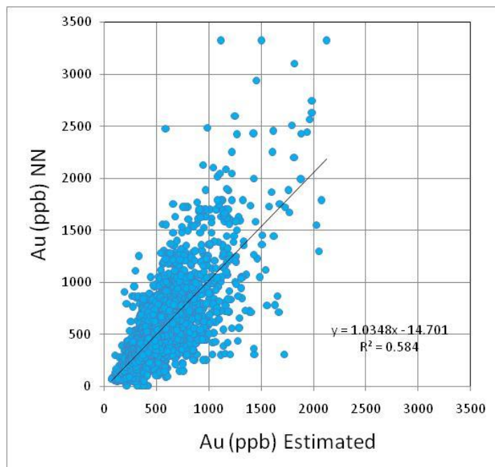
Figure 14-31: Dispersion Graph for DO (Sur, 120), All Samples
