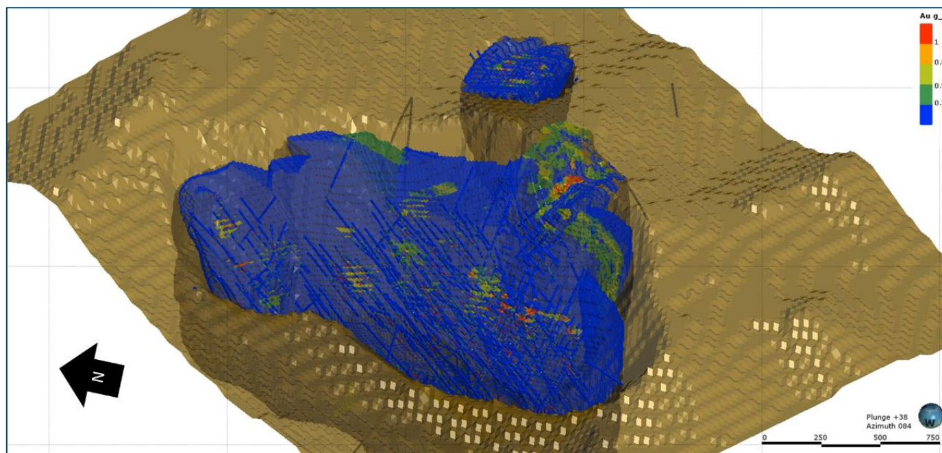
Figure 14-35: Isometric View of the Dorado Area Block Model and Base Case Optimized Pit Shell (Looking northeast)
