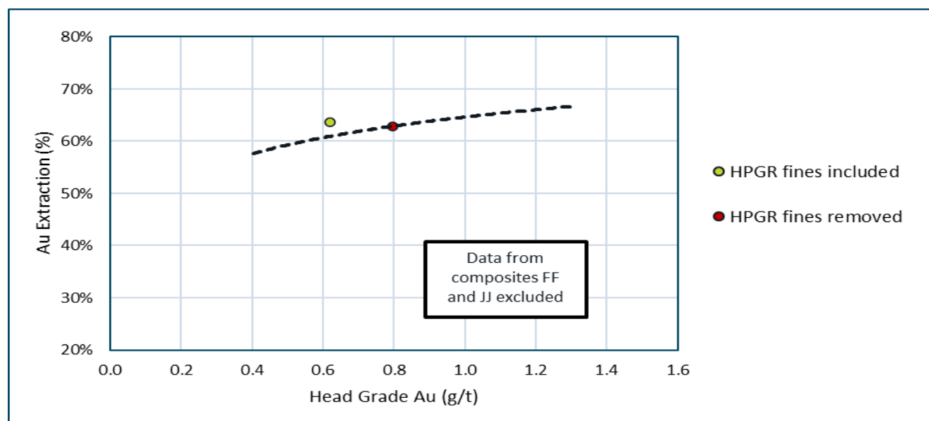
Figure 13-4: Impact of Fines Removal on Gold Leach Extraction
