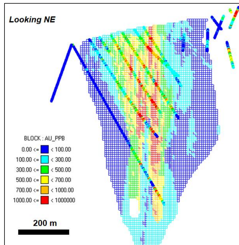
Figure 14-24: DO - Main Body – Central Zone – Vertical Section
