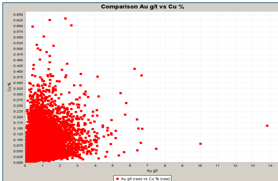
Figure 14-4: Statistical Comparison Between Gold and Copper Values, Dorado Oeste Deposit
