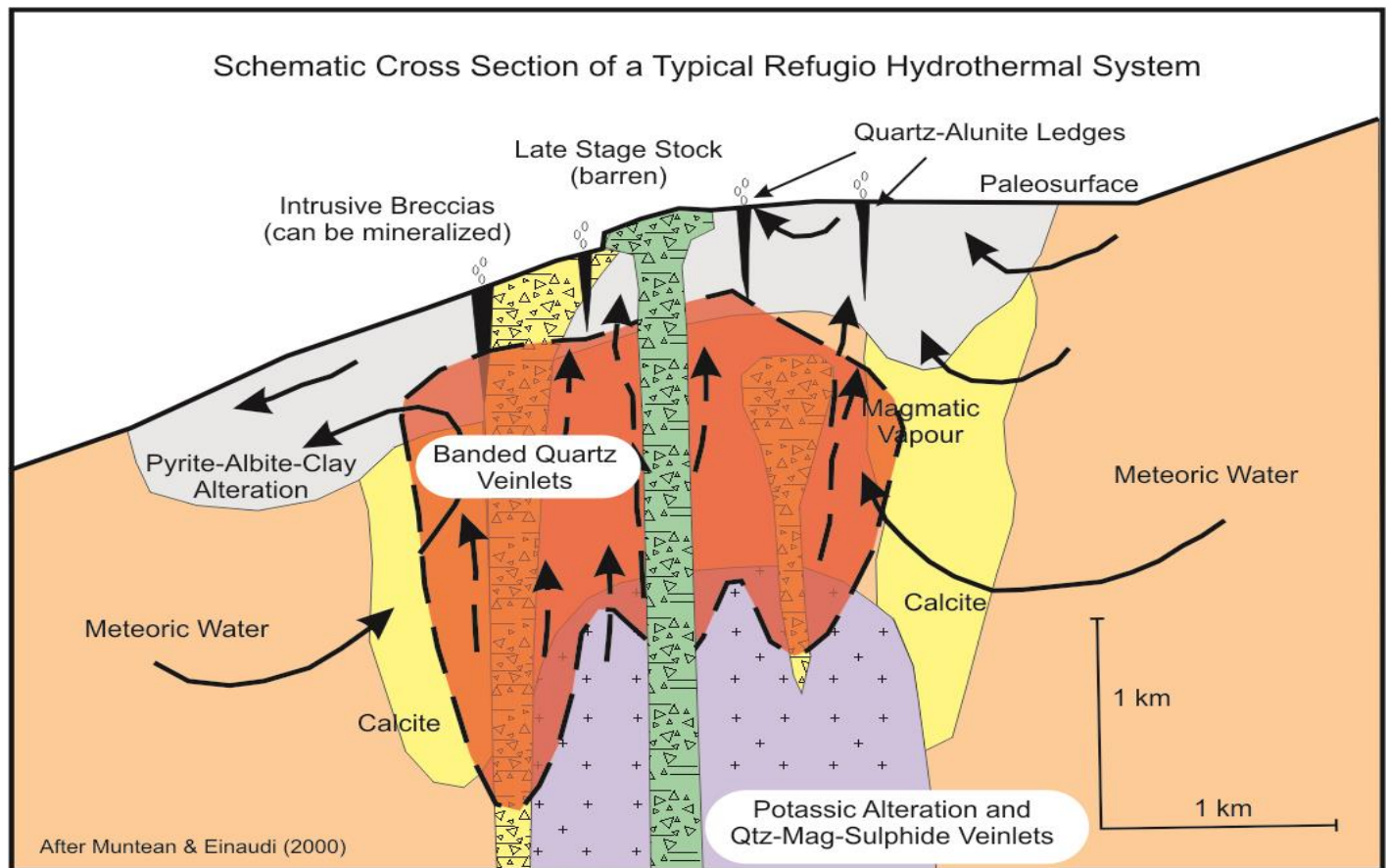
Figure 8-1: Schematic Cross-Section Showing Reconstruction of a Typical Refugio Hydrothermal System
