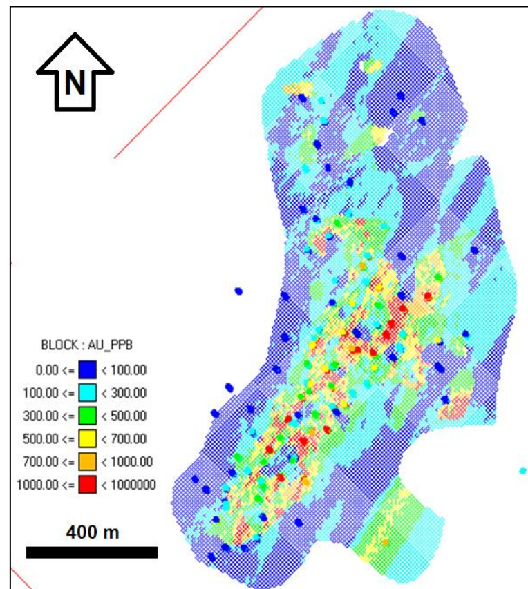
Figure 14-22: Bench Plan 4655, Dorado Block Model
