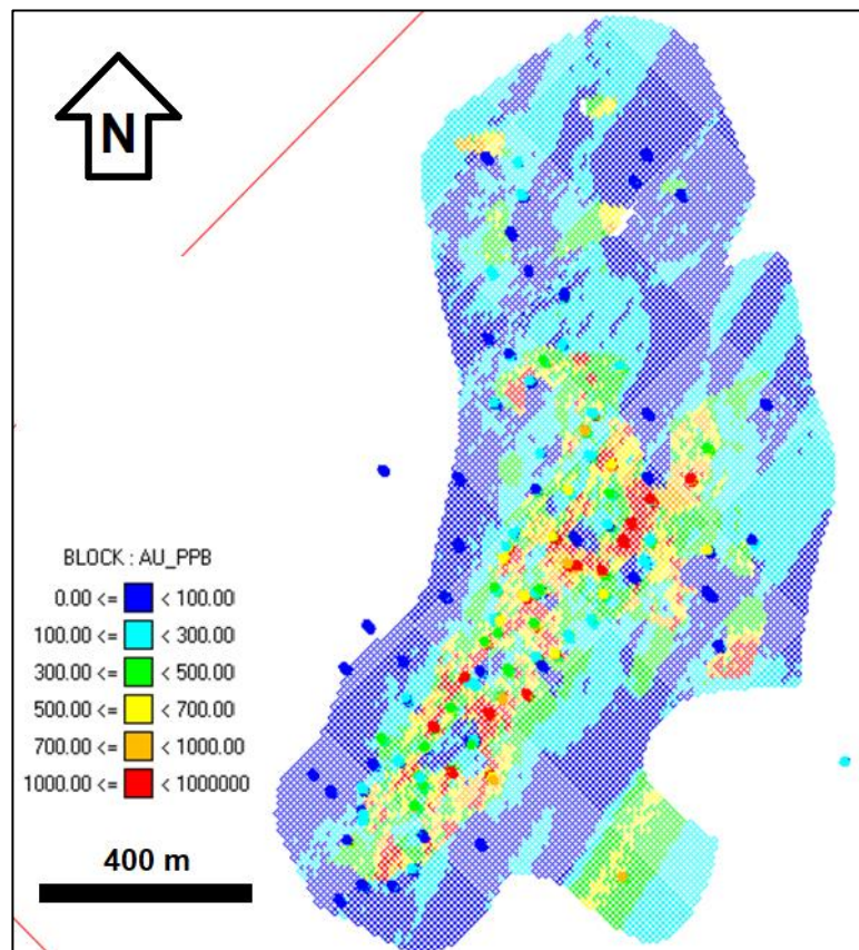
Figure 14-21: Bench Plan 4605, Dorado Block Model
