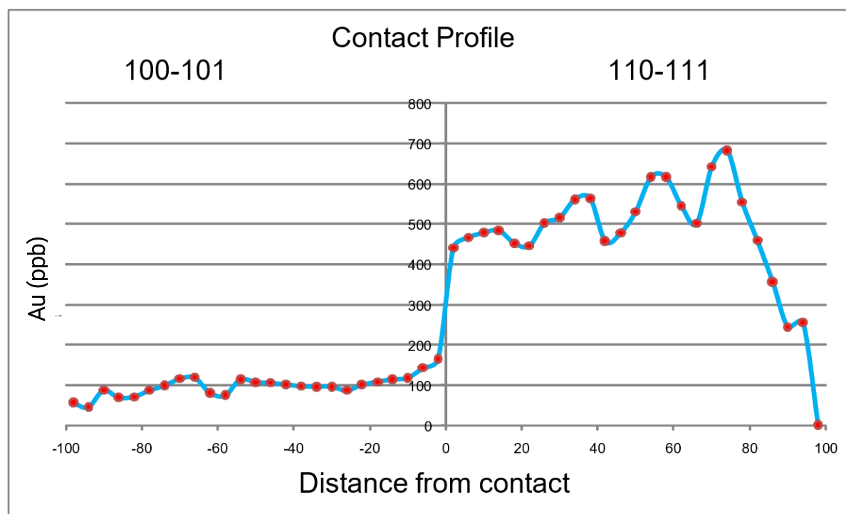
Figure 14-9: Contact Analysis, Dorado Oeste (Norte) Deposit, Domain 100/101 – 110/111
