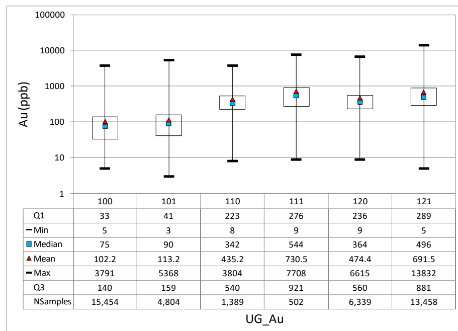
Figure 14-8: Box-and-Whisker Plot of Gold Assays Contained Within the Geological Domains (Columns), Including Ungrouped Weights (Samples ≥ 1m)
