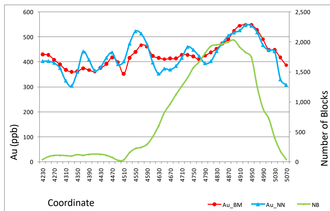
Figure 14-27: Drift Analysis for the DO (Norte) Domain (Code 100/101) (Bench data are presented on the y-axis while cross-sectional data are presented on the x-axis)
