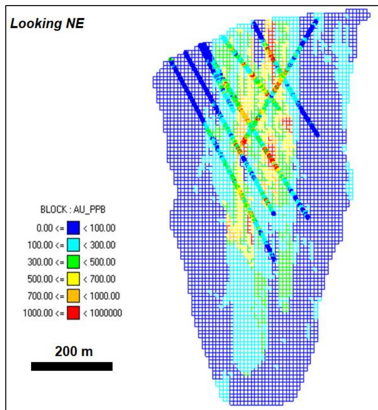
Figure 14-23: DO - Main Body – South End – Vertical Section
