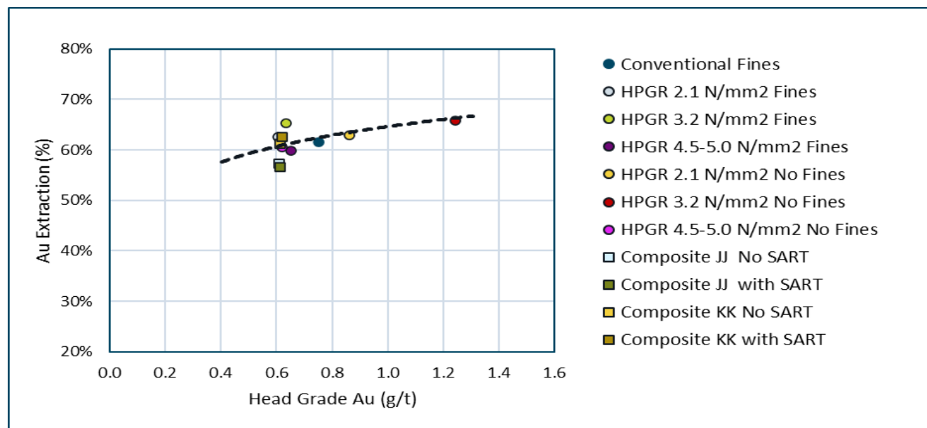
Figure 13-3: Impact of Process Variables on Gold Leach Extraction
