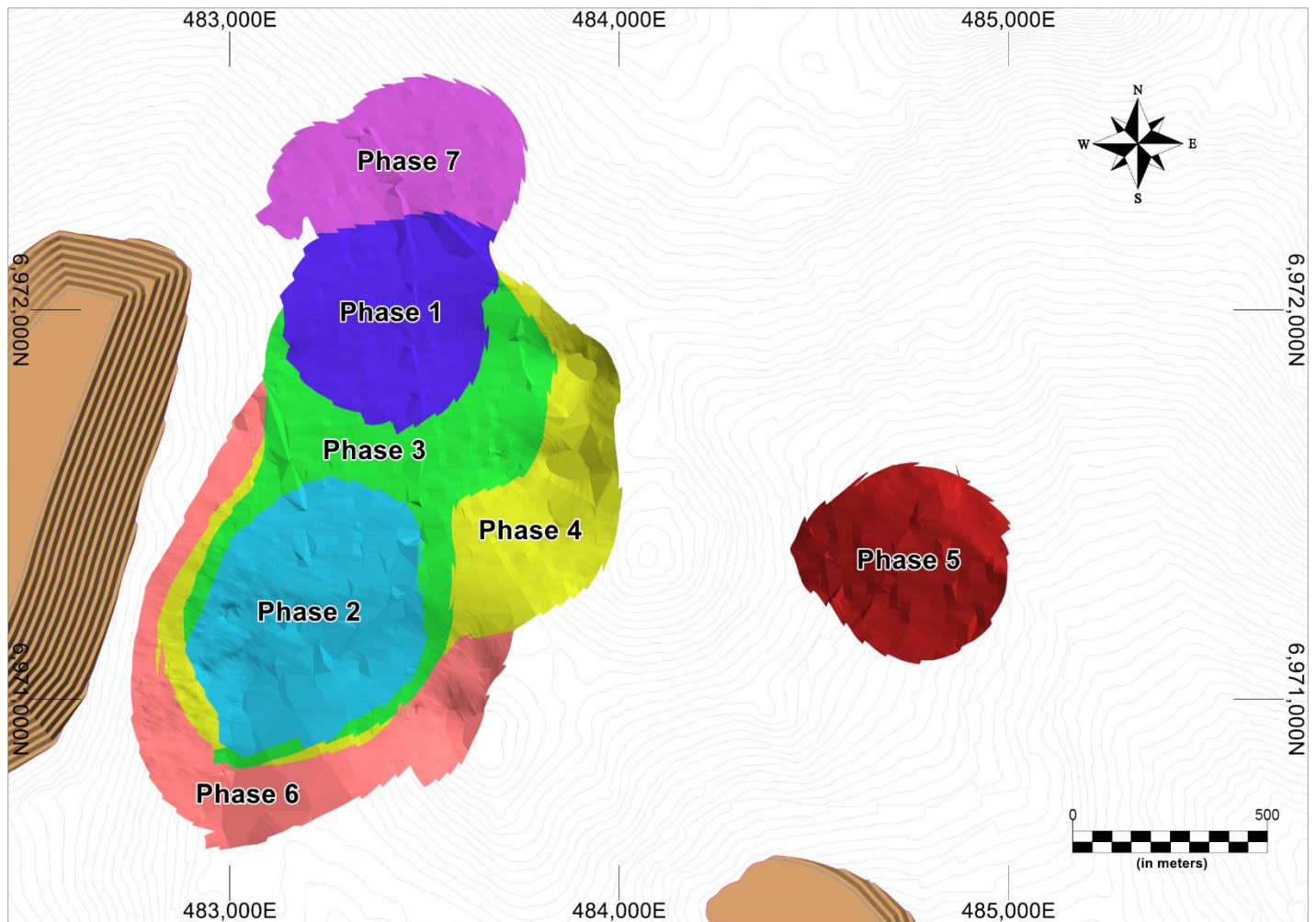
Figure 16-5: Pushbacks
